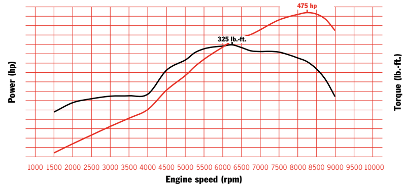
911 GT3: 475 hp at 8,250 rpm, 325 lb.-ft. at 6,250 rpm
