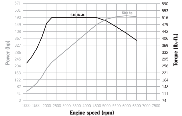
Cayenne Turbo: 516 lb.-ft. between 2250 and 4500 rpm, 500 horsepower at 6000 rpm
