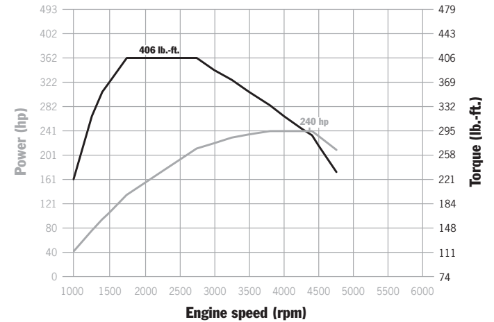
Cayenne Diesel: 406 lb.-ft. between 1750 and 2500 rpm, 240 horsepower between 3800 and 4400 rpm
