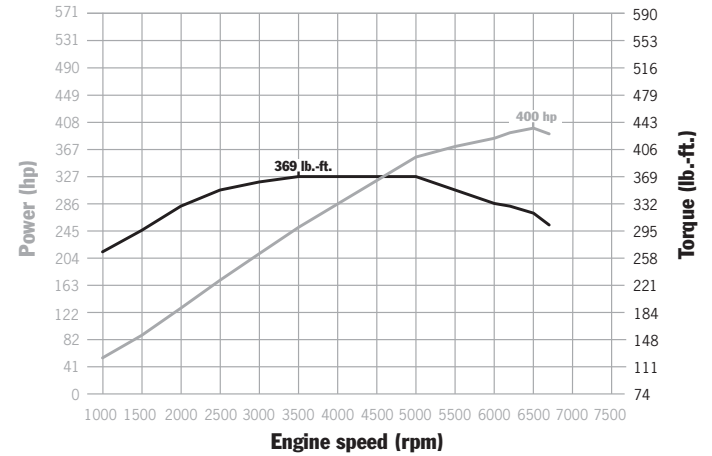
Cayenne S: 369 lb.-ft. at 3500 rpm, 400 horsepower at 6500 rpm
