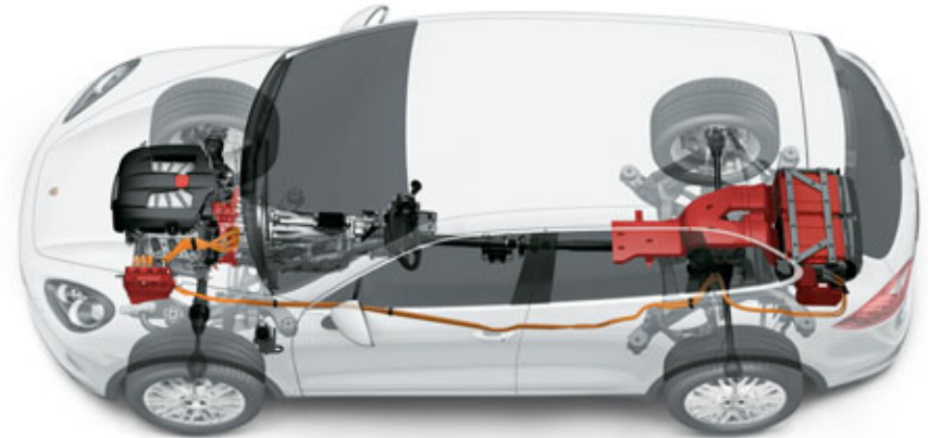
Parallel Full Hybrid drivetrain
